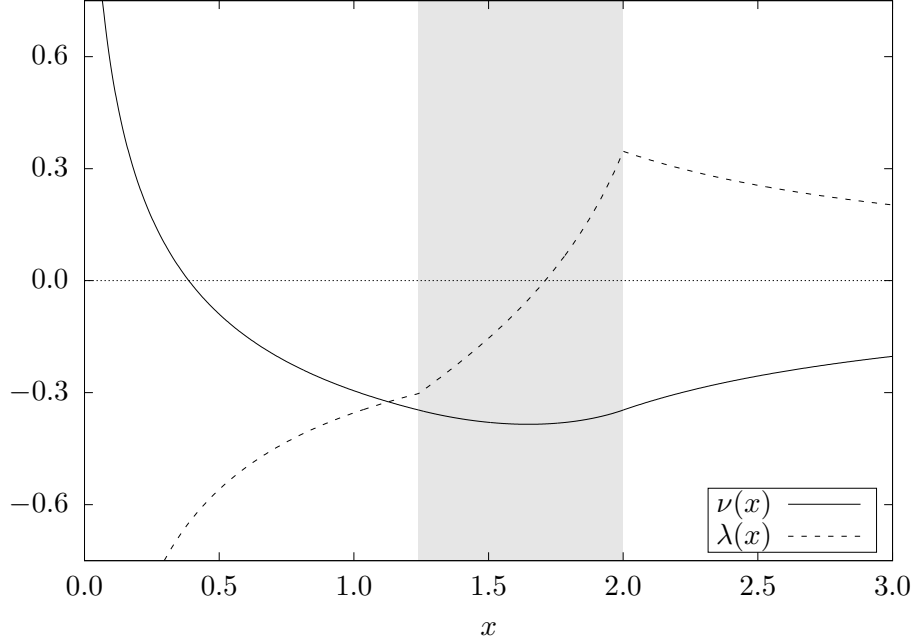
Figure 4: The functions \nu(x) and \lambda(x) for \eta = 5.0 , x_2 = 2.0 and x_M = 1.0 . The shaded area indicates the matter region, to its right is the outer vacuum and to its left is the inner vacuum. Here we have x_1 = 1.24050 and x_\mu = 1.03035 .
