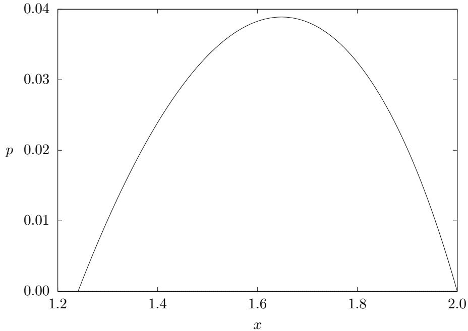
Figure 3: The dimensionless pressure p calculated numerically for \eta = 5.0 , x_2 = 2.0 and x_M = 1.0 . Here we have x_1 = 1.24050 and x_\mu = 1.03035 .
