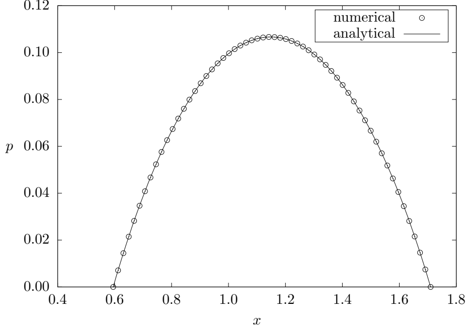
Figure 1: Comparison between the dimensionless pressure p(x) calculated analytically and numerically using the Runge-Kutta fourth-order algorithm for \eta = 2.0 , x_2 = 5^{1/3} and x_M = 1.0 , resulting in x_1 = 0.594881 and x_\mu = 0.596494 .
