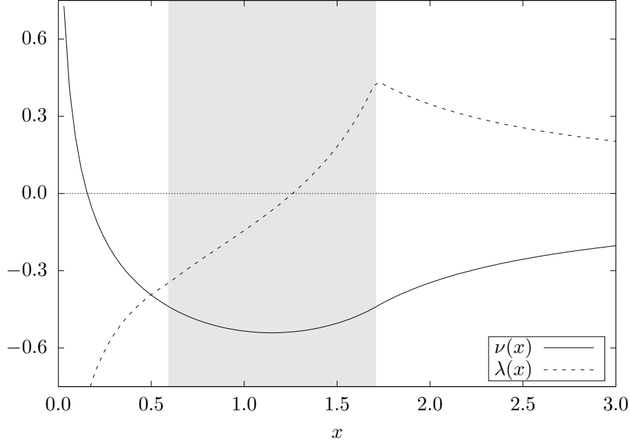
Figure 2: The functions \nu(x) and \lambda(x) for \eta = 2.0 , x_2 = 5^{1/3} and x_M = 1.0 . The shaded area indicates the matter region, to its right is the outer vacuum and to its left is the inner vacuum. Here we have x_1 = 0.594881 and x_\mu = 0.596494 .
